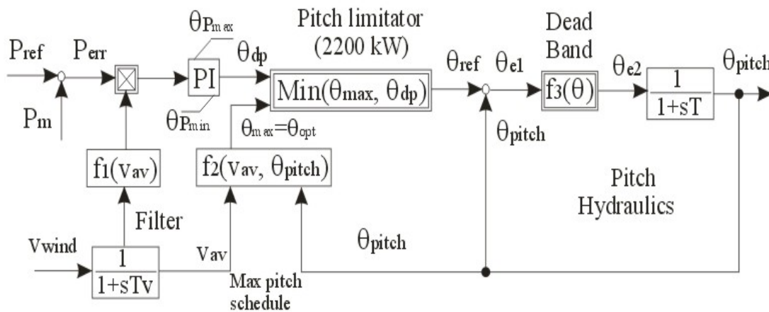
Fig. 4. The block diagram of blade pitch angle control system [20].
