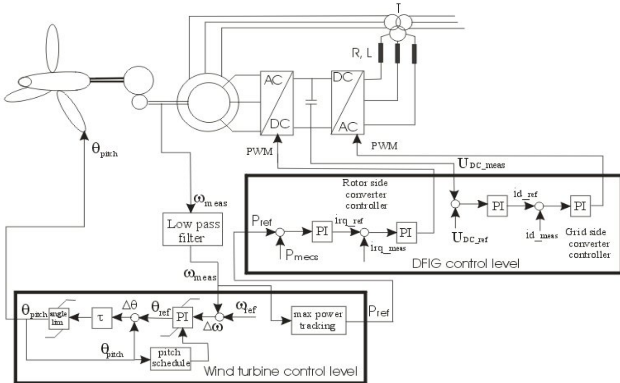
Fig. 8. An overview of the variable-speed wind turbine control strategy.
