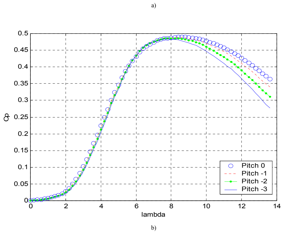
Fig. 5. Power coefficient ( C_p ) of a 2MW wind turbine versus wind speed (a), and the tip speed ratio ( \lambda ), (b) at different pitch angles.
