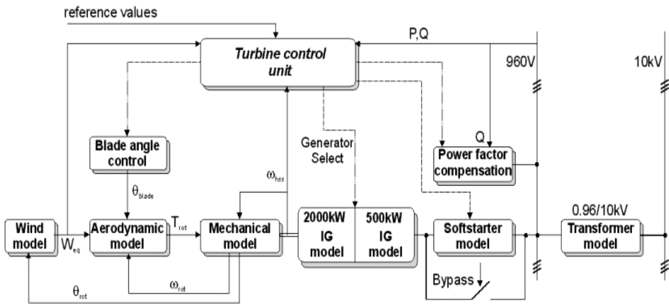
Fig. 3. Block diagram of an active stall controlled wind turbine with constant speed using a cage-rotor induction generator [17].
