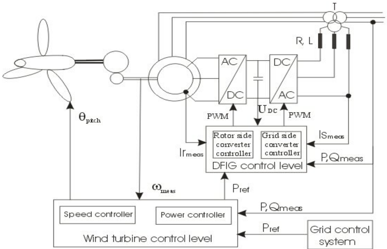
Fig. 7. The control system of a variable-speed wind turbine with DFIG fed by a back-to-back VSI.
