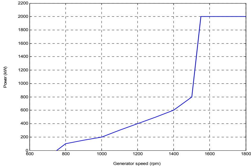
Fig. 6. Electrical power versus generator speed characteristic used in the maximum power tracking controller.
