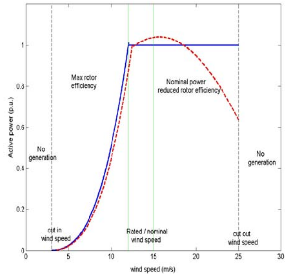
Fig. 2. Typical power curves and operation areas of a stall (dashed line) and pitch controlled (solid line) wind turbines
