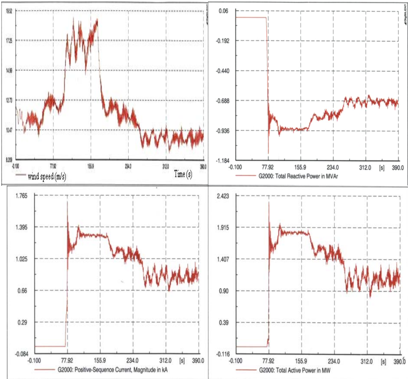
Fig. 10. Simulation results during sudden changes in wind speed for a 2MW active stall constant-speed wind turbine using CRIG.
