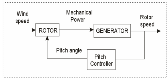
Fig. 1. Rotor speed control principle for wind speeds above nominal.
