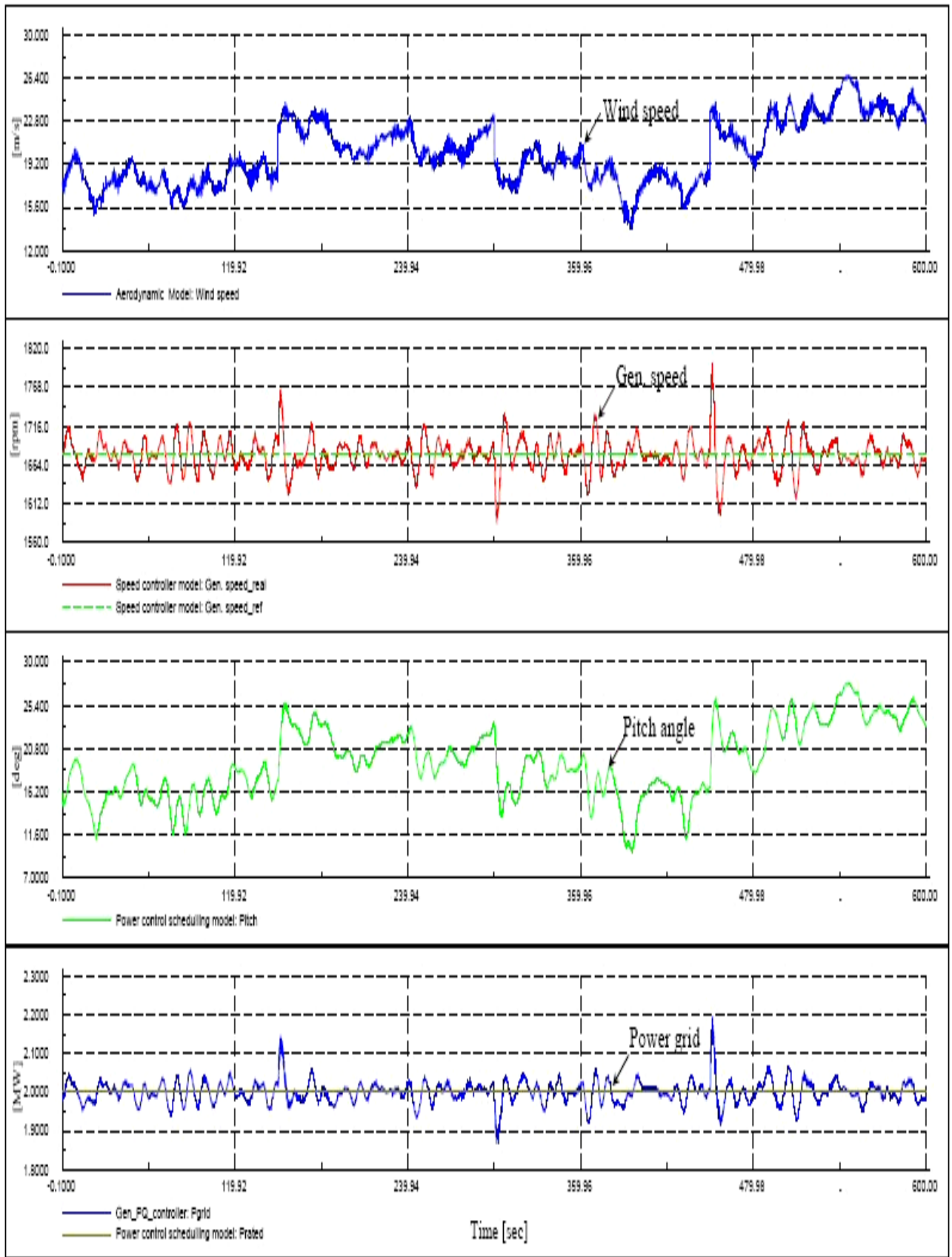
Fig. 9. Simulation results during sudden changes in wind speed for a 2MW pitch controlled variable-speed wind turbine using DFIG.
