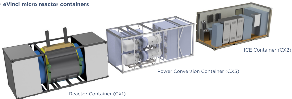
fig. 2 eVinci micro reactor containers
