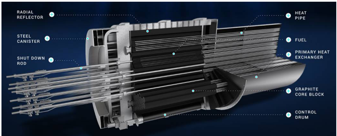
fig. 1 eVinci micro reactor core
