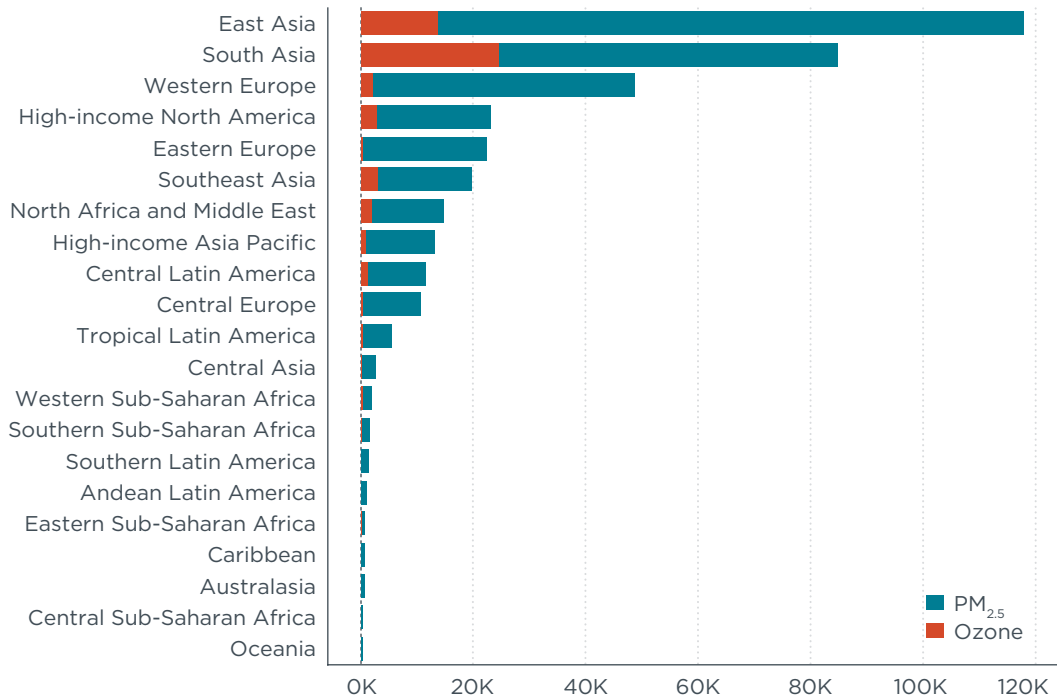
Figure 6. Total number of transportation-attributable PM 2.5 and ozone deaths in 2015 by world region.
