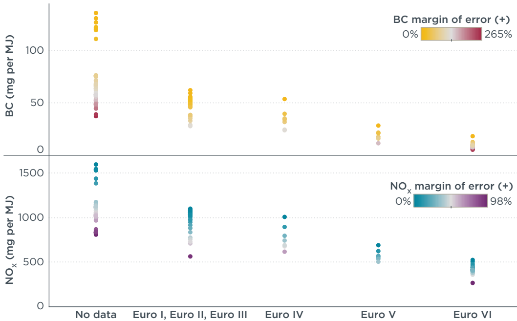
Figure A1. Average estimated fuel-specific BC and NO x emission factors for diesel road transport in 2015. Countries are grouped according to their latest emissions standard implemented for new heavy-duty trucks as of 2015.
