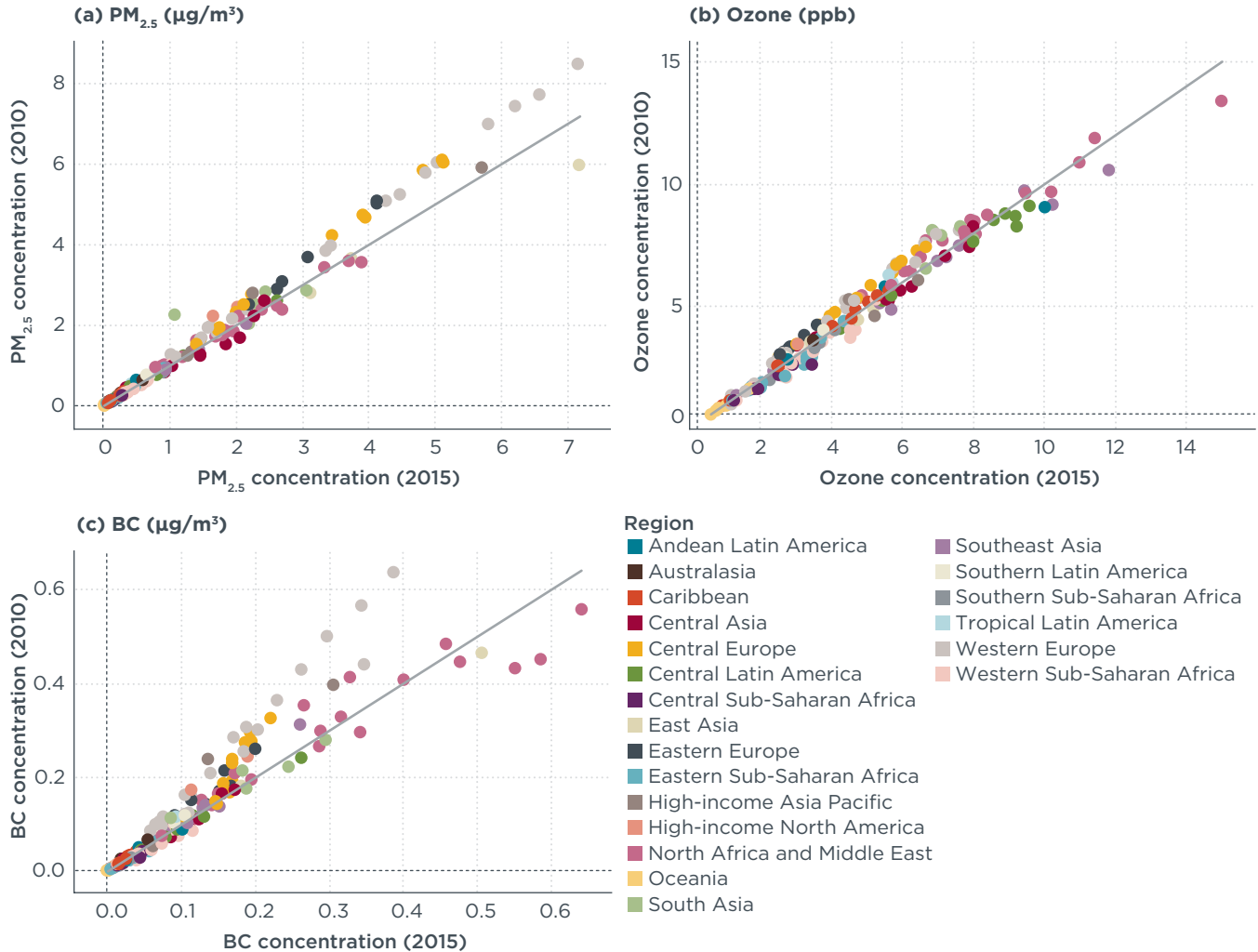
Figure 5. Scatterplots of annual average PM 2.5 , 6-month average of the 8-hour daily maximum ozone, and annual average black carbon (BC) concentrations in 2010 versus 2015 by country.
