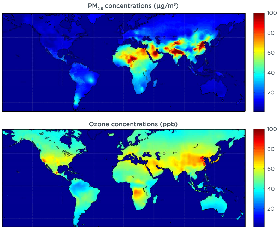
Figure 1. Total PM_{2.5} (annual average) and ozone concentrations (6-month average of the 8-hour daily maximum) in 2010. PM_{2.5} concentrations are from Shaddick et al. (2018). Ozone concentrations are from Chang et al. (2018). Maximum concentrations globally are 387 \mu\text{g}/\text{m}^3 for PM_{2.5} and 94 ppb for ozone.
