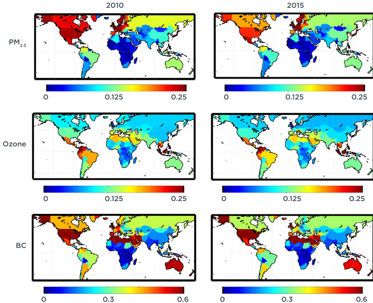
Figure 3. National population-weighted TAF (unitless) for PM_{2.5} , ozone, and BC in 2010 and 2015. BC TAFs are estimated from simulated concentrations because we did not estimate BC-specific mortality separately from PM_{2.5} mortality.
