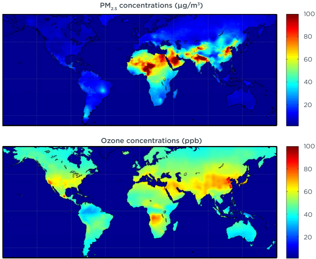
Figure 2. Total PM_{2.5} (annual average) and ozone concentrations (6-month average of the 8-hour daily maximum) in 2015. PM_{2.5} concentrations are from Shaddick et al. (2018). Ozone concentrations are from Chang et al. (2018). Maximum concentrations globally are 329 \mu\text{g}/\text{m}^3 for PM_{2.5} and 94 ppb for ozone.
