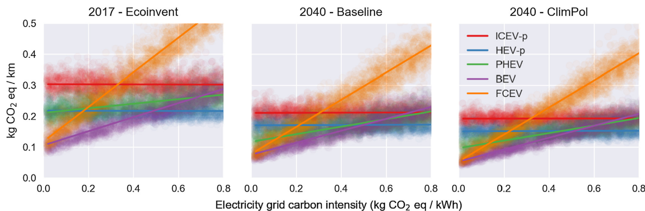
Fig. 9. Life cycle climate change impacts of lower medium size passenger vehicles shown for different electricity grid carbon intensities. Hydrogen is assumed to be produced using electrolysis with grid electricity. The cloud of dots represents the actual Monte Carlo analysis results, while the solid lines represent lines fit to the data to improve visibility.
