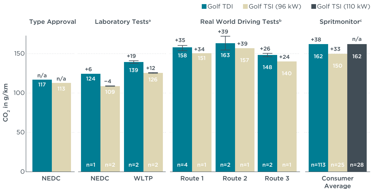
Figure 1: CO 2 levels of the Golf TDI (diesel) and Golf TSI (gasoline). Comparison of test results with declared type approval values (left-hand side) and Spritmonitor consumer reported numbers (right-hand side). The error bars show the minimum to maximum range of results if multiple tests were performed. The number of tests is shown at the bottom of each bar. The ratio of CO 2 emission level vs type approval value is shown above each bar.
