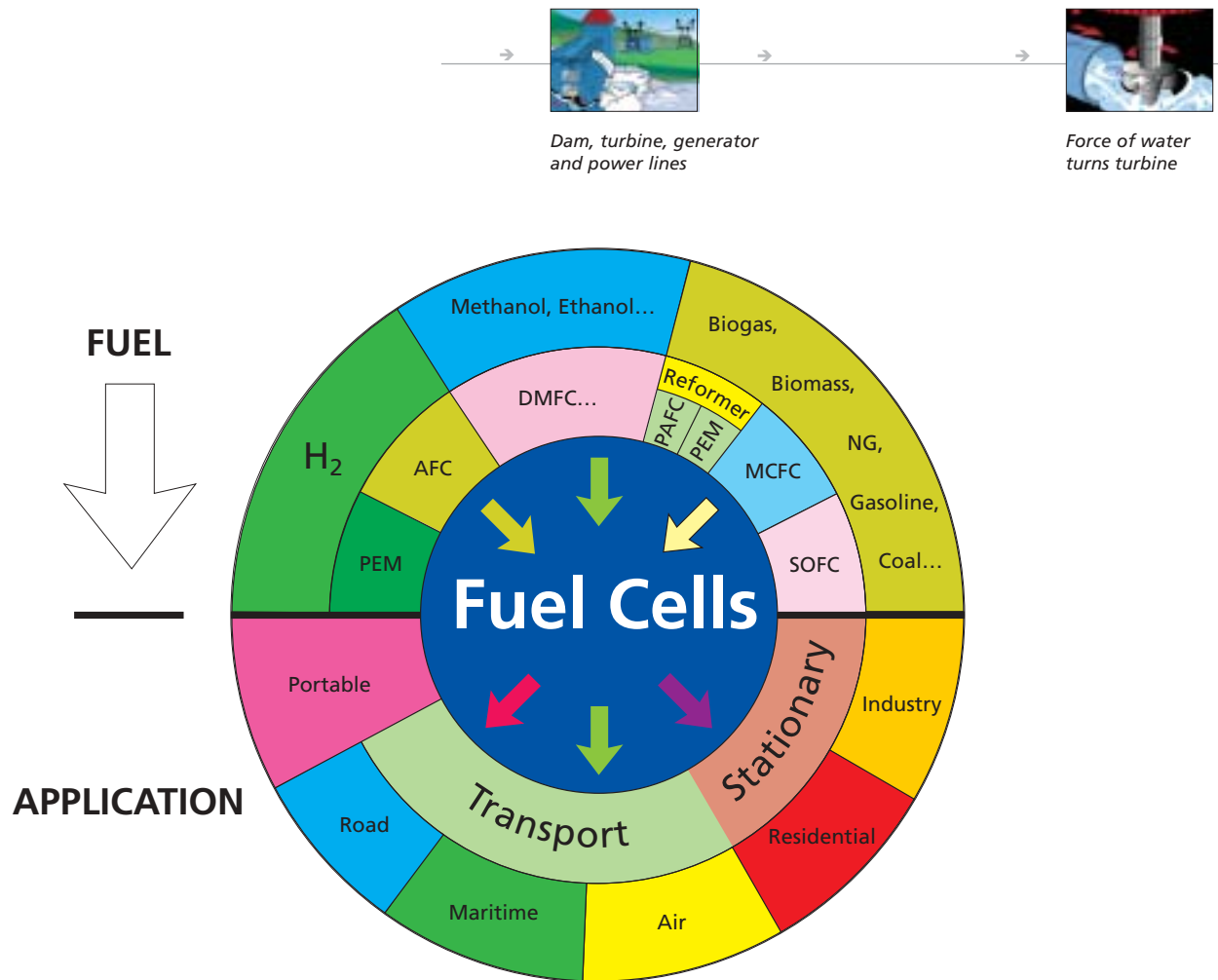
Figure 2: Fuel cell technologies, possible fuels and applications
