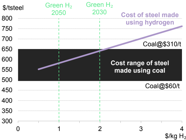
Figure 8: Levelized cost of steel: hydrogen versus coal
