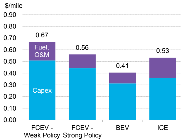
Figure 9: Total cost of ownership of SUVs in the U.S., 2030
